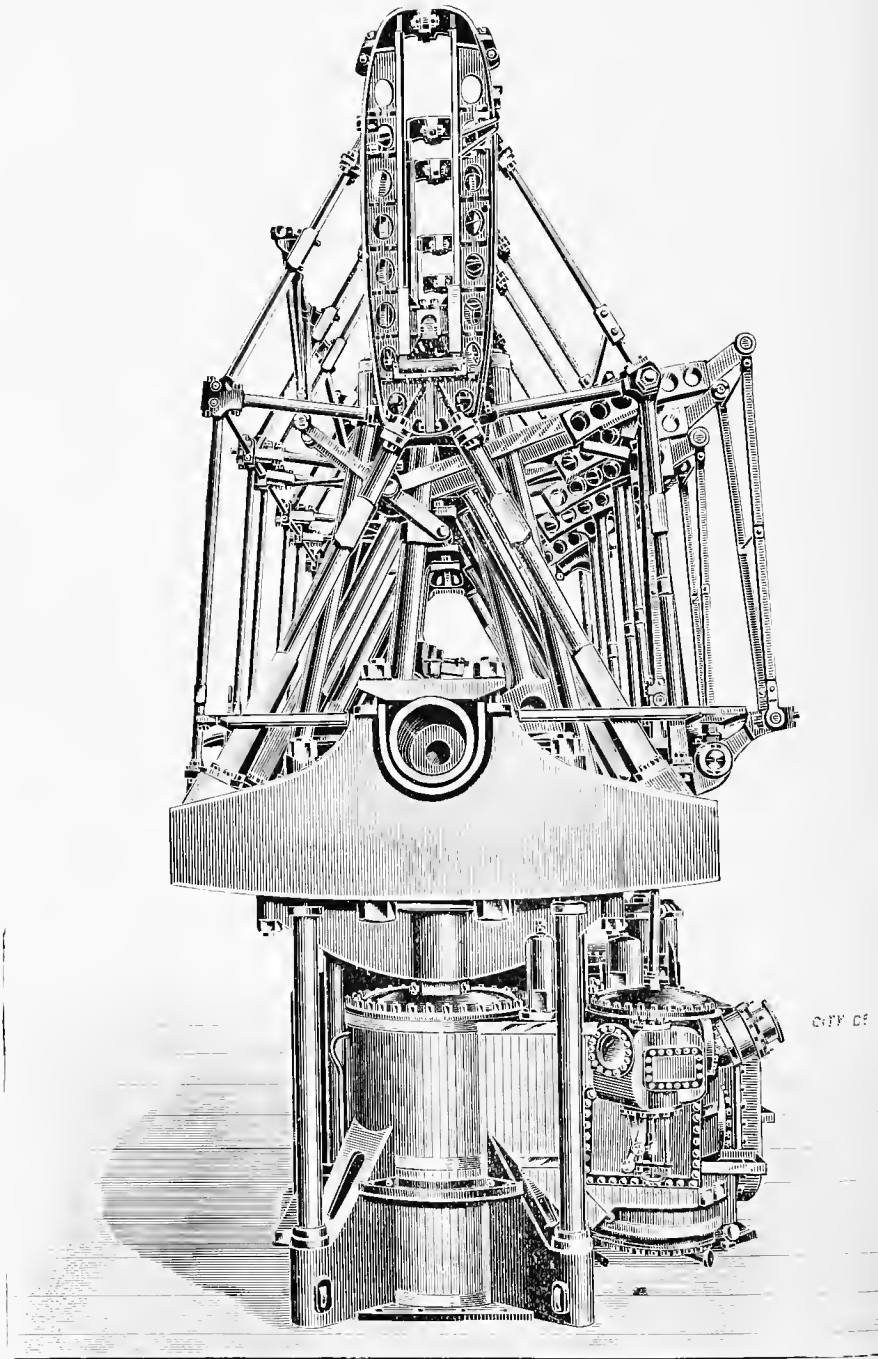
STEEPLE ENGINES OF THE HOLYHEAD & DUBLIN MAIL STEAMER BANSHER.
